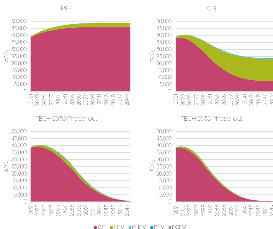
Figure 6.2 Annual stock tailpipe CO 2 emissions (KtCO 2 )
