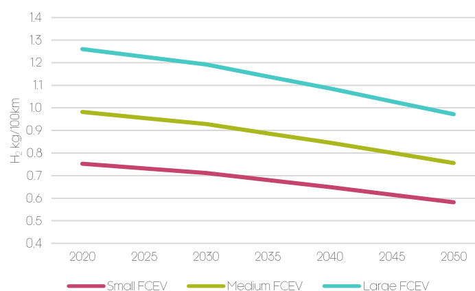
Figure 3.4 Fuel consumption assumptions for small, medium, and large FCEVs ( H_2 kg/100km)
