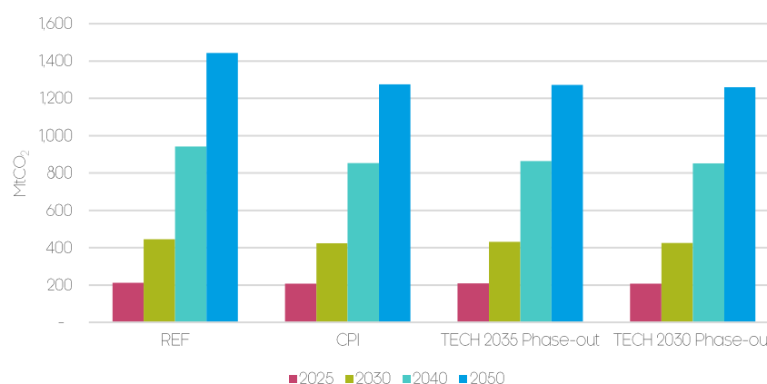
Figure 7.3: Cumulative CO 2 well-to-wheel emissions reductions compared to the baseline scenario ('Central' power sector scenario)
