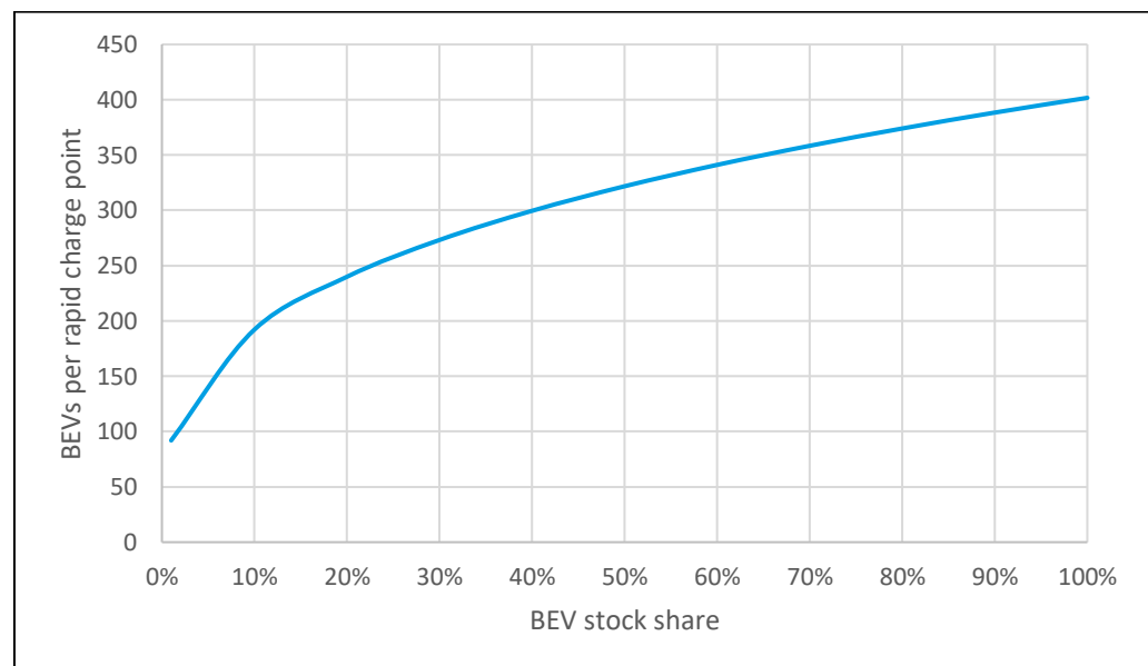
Figure 0.3: Number of BEVs per rapid charge point as a function of BEV stock share 16
