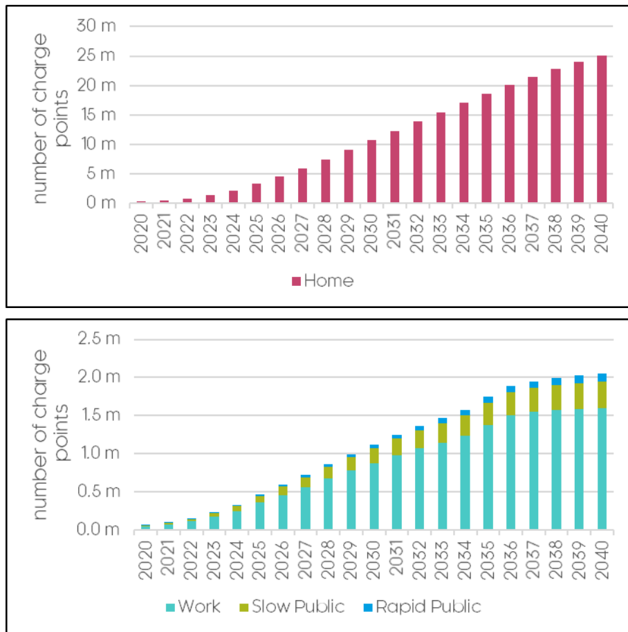
Figure 2.8: Number of charge points required with 2035 ICE Phase Out
