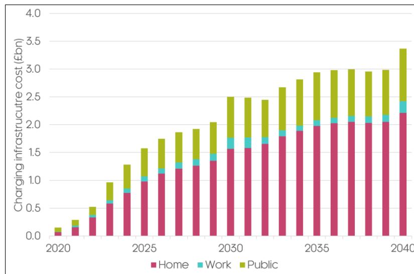
Figure 2.11: Annual charging infrastructure investment cost under 2030 ICE Phase Out
