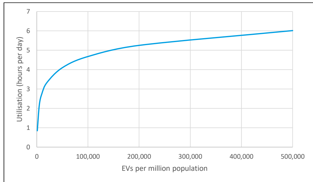
Figure 0.2: Average utilisation per day for slow public charge points (3-22kW) as a function of EVs per million population 16
