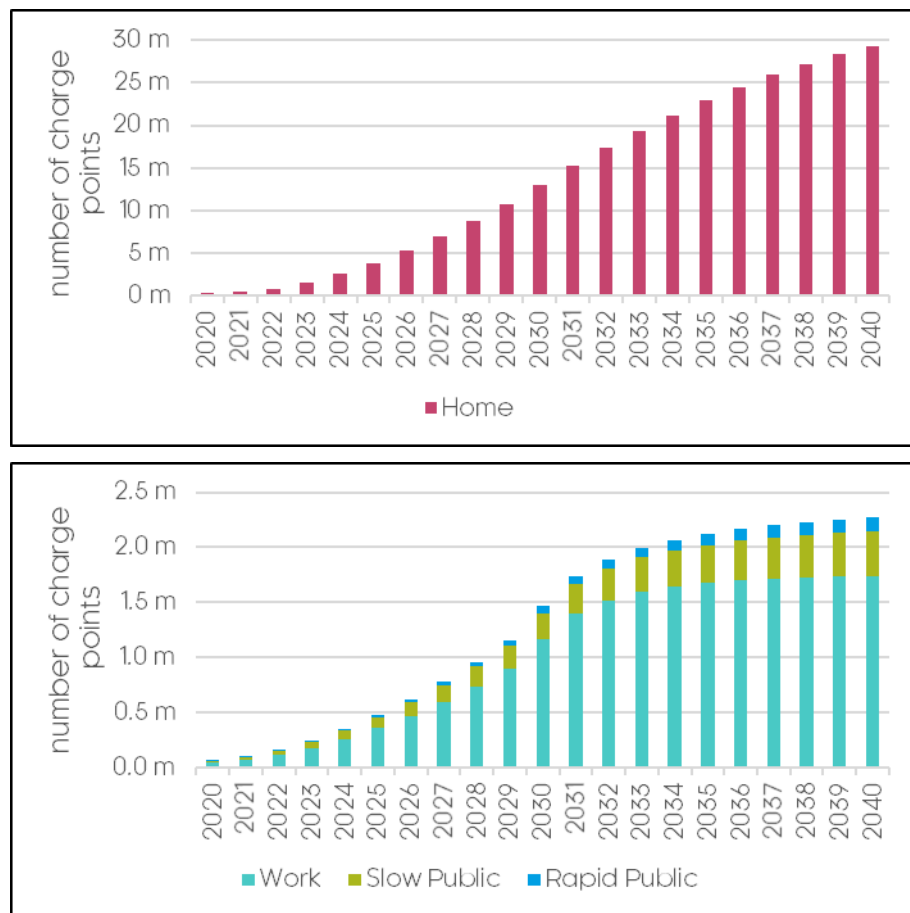
Figure 2.9: Number of charge points required with 2030 ICE Phase Out
