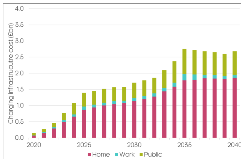
Figure 2.10: Annual charging infrastructure investment cost under 2035 ICE Phase Out
