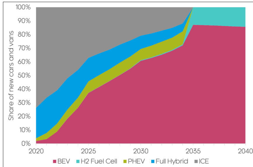
Figure 2.2 Powertrain share of new cars and vans 2020-2040, under the 2030 ICE Phase Out scenario
